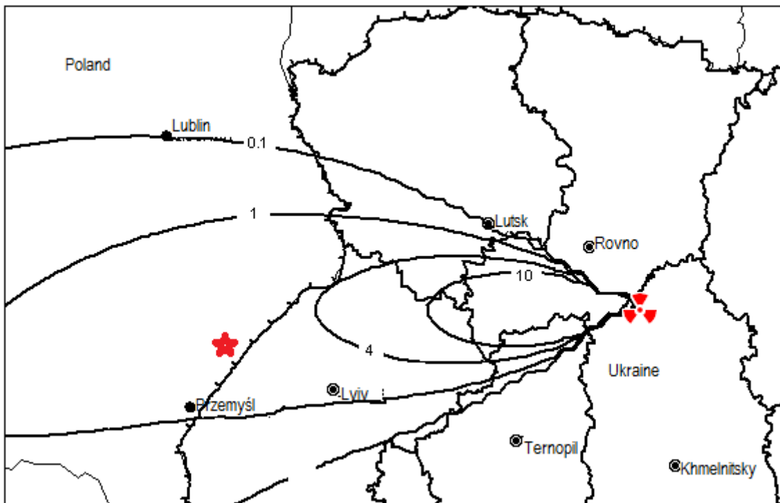
Figure 2.3 – Isolines of the density field of the fallouts ^{131}\text{I} ( \text{Bq}\cdot\text{m}^{-2} ) under MDBA at KNPP (meteorological scenario 2)
