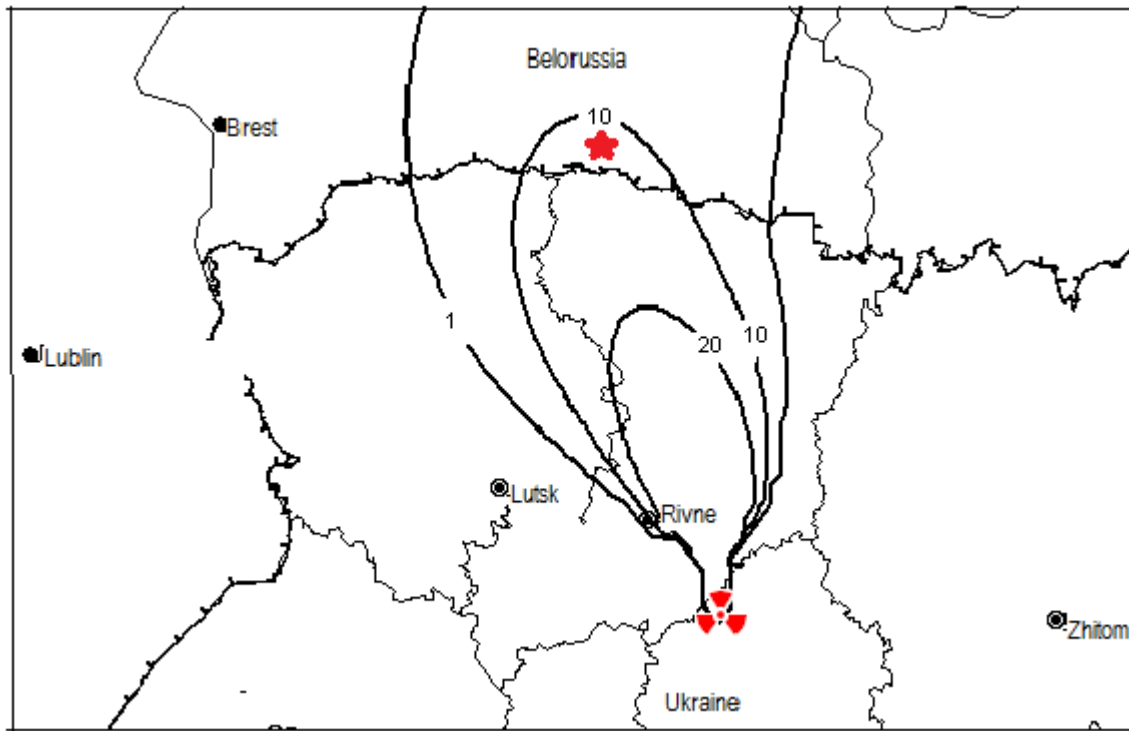
Figure 2.1 – Isolines of the density field of the fallouts ^{131}\text{I} ( \text{Bq}\cdot\text{m}^{-2} ) under maximum design-basis accident at KNPP (meteorological scenario 1)
