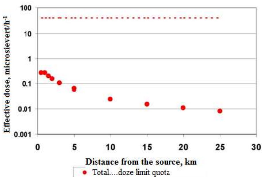
Figure 1.1– Dependence of the radiation doze for the reference group of population on gas and aerosol releases from the source (normal operation)
