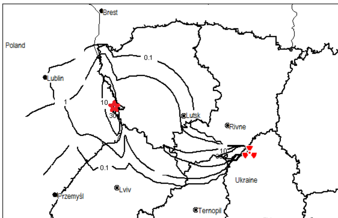
Figure 2.6 – Isolines of the density field of the fallouts ^{131}\text{I} ( \text{Bq}\cdot\text{m}^{-2} ) under MDBA at KNPP (meteorological scenario 3A)
