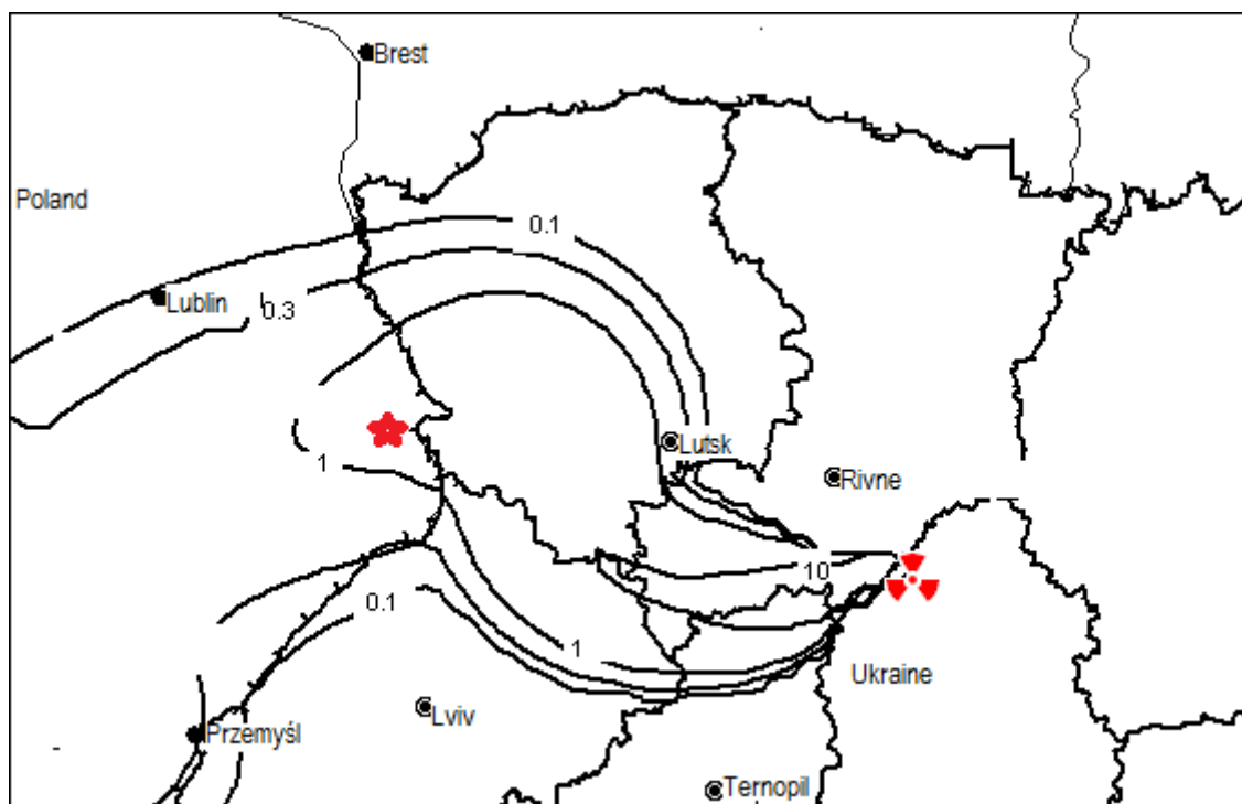
Figure 2.5 – Isolines of the density field of the fallouts ^{131}\text{I} ( \text{Bq}\cdot\text{m}^{-2} ) under MDBA at KNPP (meteorological scenario 3)
